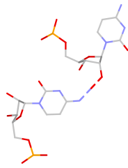
C:C pfS(sb:O2*-N4)
