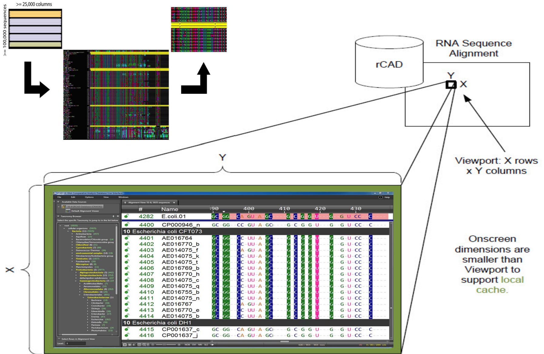
rCAD User Interface (rCAD-UI) Alignment Visualization
