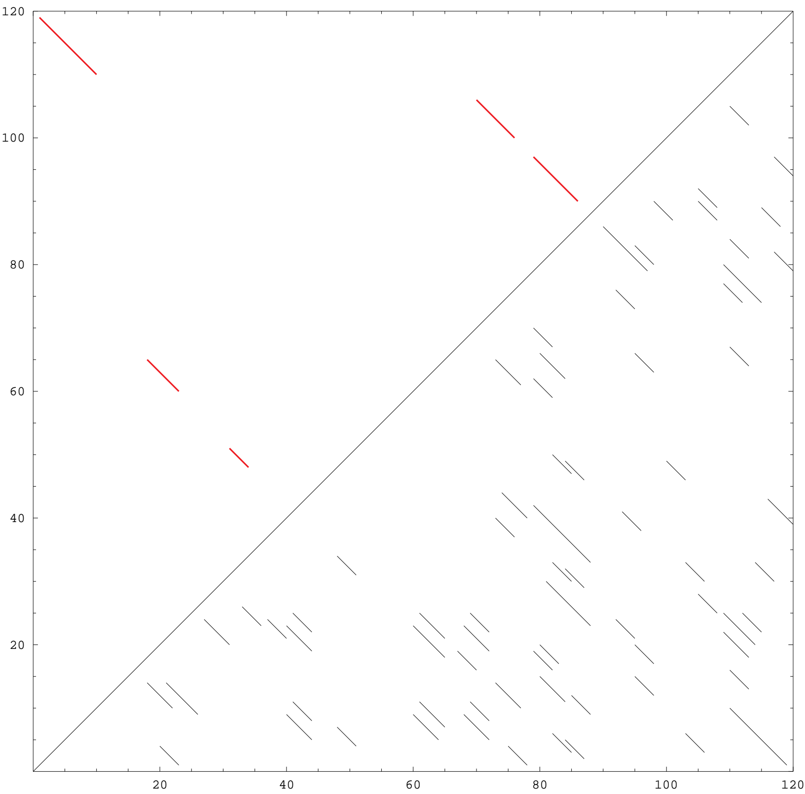
5S rRNA -- All Possible Helices
