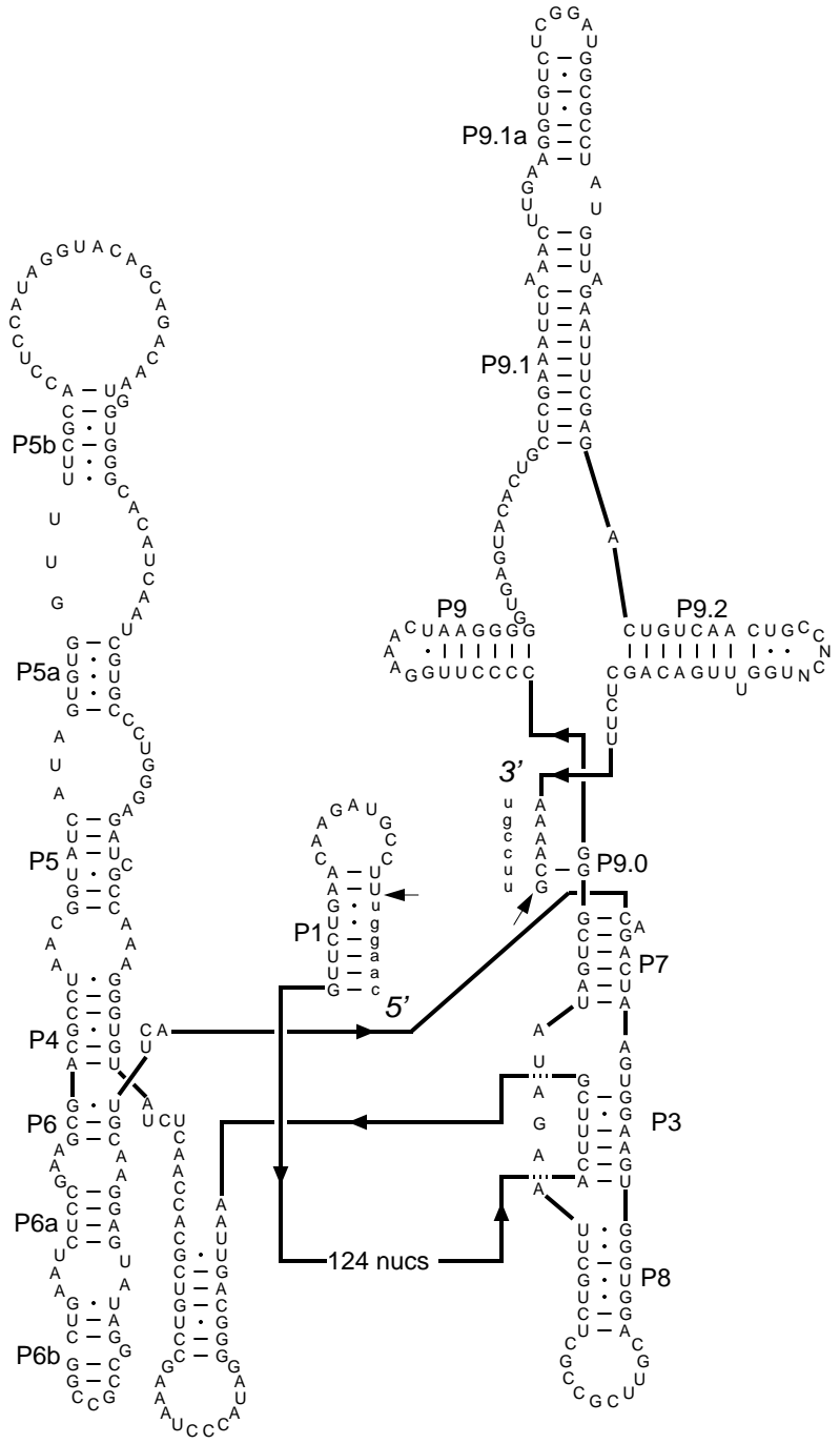
Cenococcum geophilum SSU rRNA (1506) GenBank# Z11998 Eucarya, Fungi, Ascomycota (UNK) Aug 21, 1996
