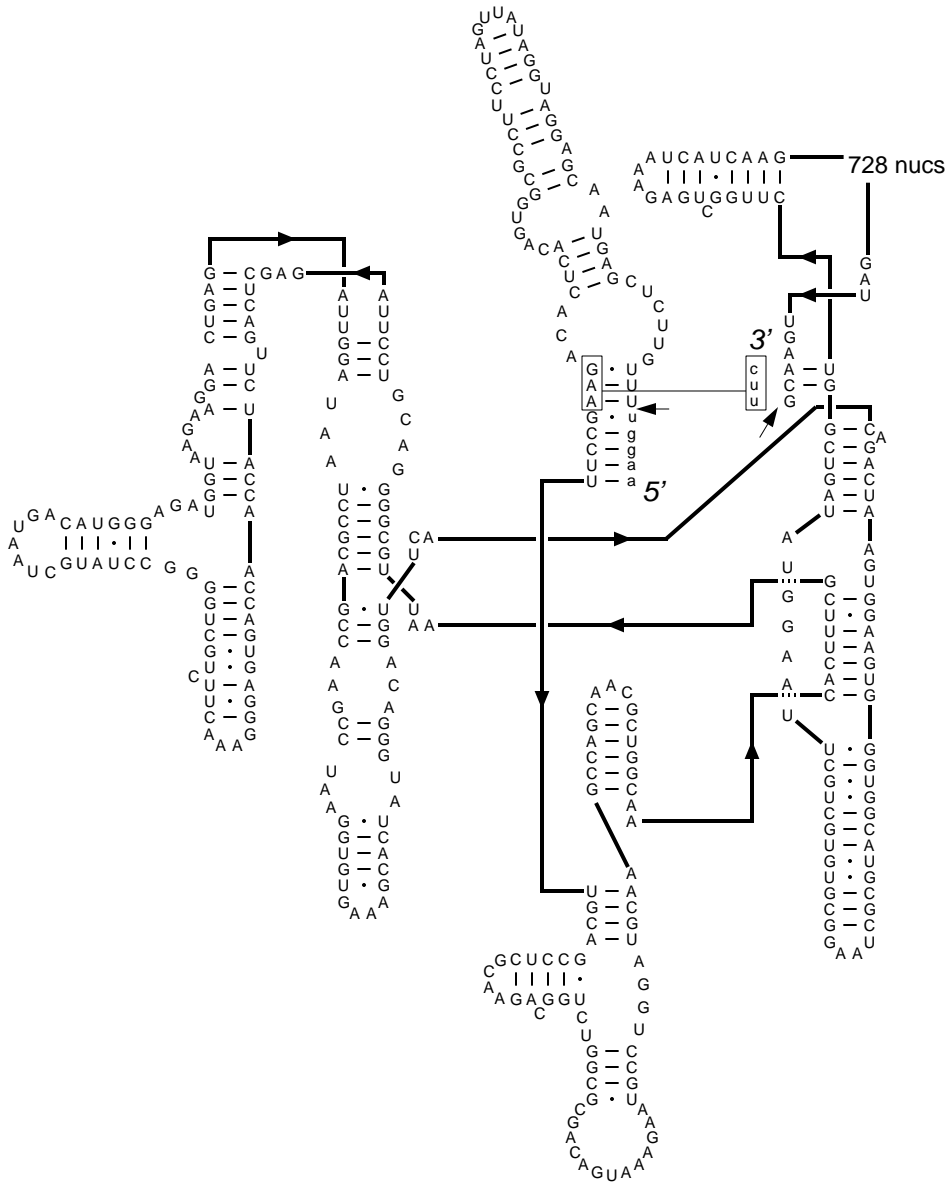
Protomyces pachydermus SSU rRNA (1506) [i2] GenBank# D85142 Eucarya, Fungi, Ascomycota (IC1) Jul 3, 1996
