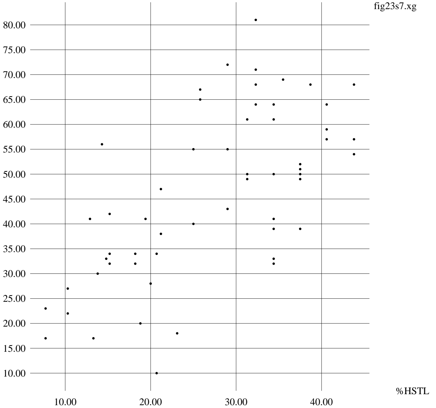
Figure 7, 16S rRNA case: score-1 vs % hairpin loops that are stable tloops
