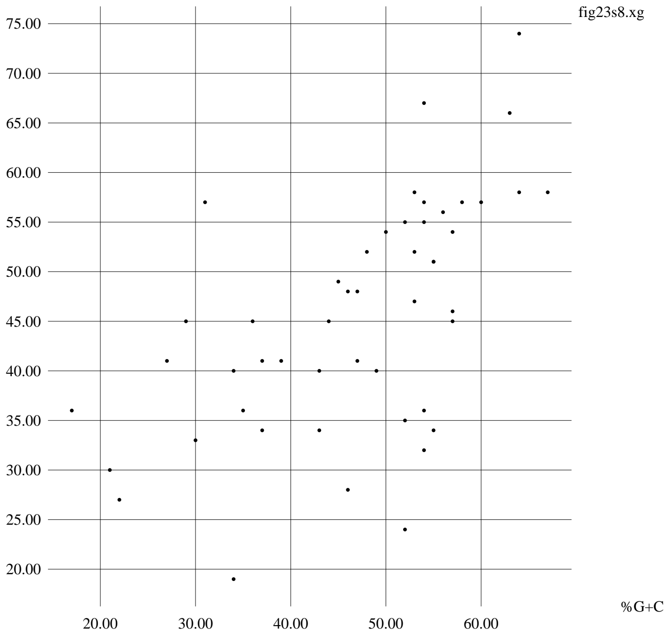
Figure 8, 23S rRNA case, no Eucarya included: score-1 vs % of G+C
