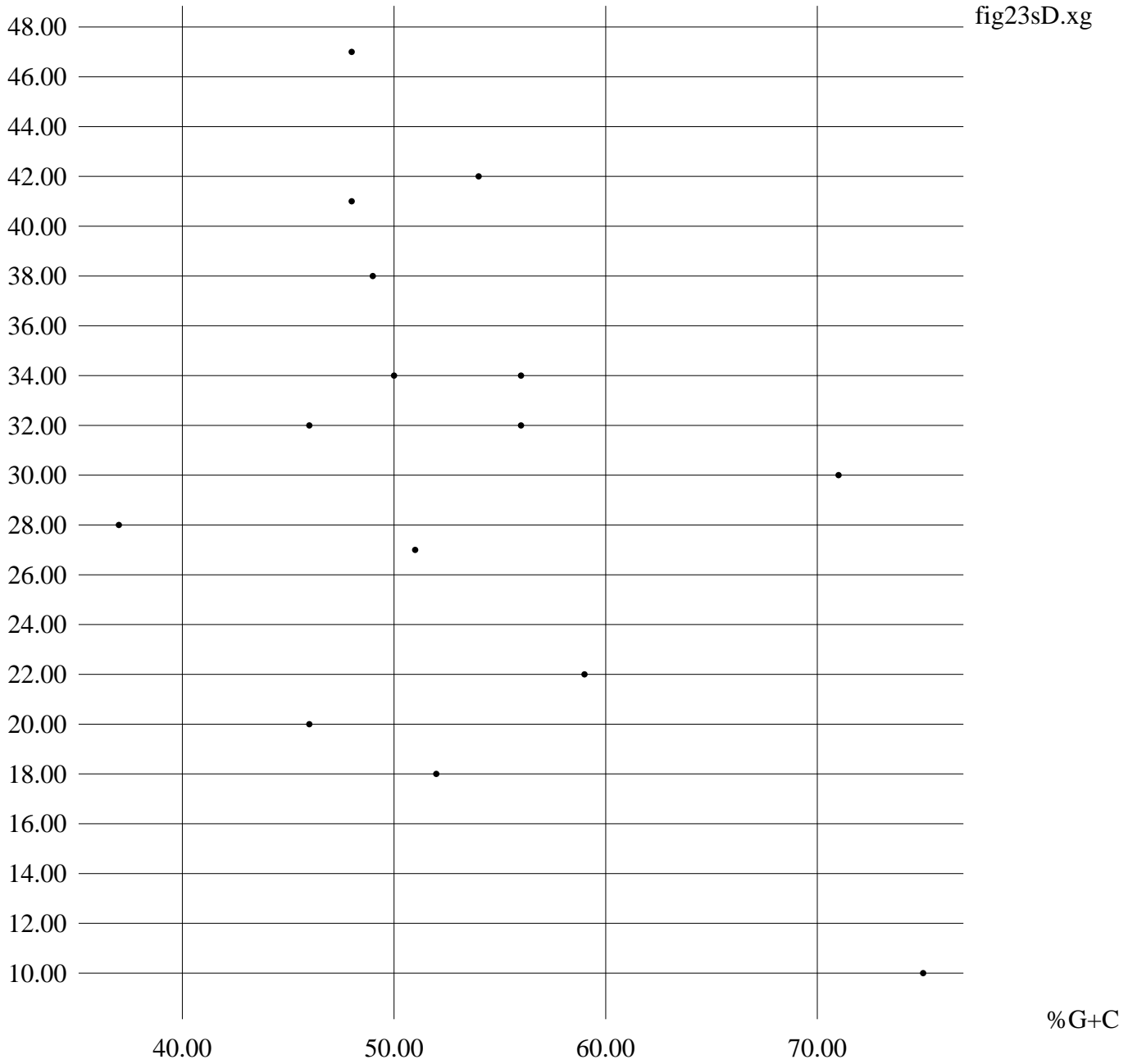
Figure D, 16S rRNA case, Eucarya only: score-1 vs % of G+C
